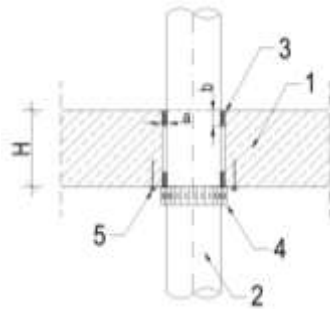
Fig. D7. Plastic pipe, MLC pipe and composite pipe without insulation penetration seals made with use of INTU FR COLLAR L SLIM collars (one-sided) in rigid floor
