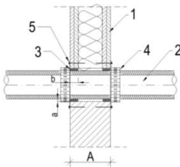
Fig. D2. Metal pipe with flexible elastomeric foam (FEF) insulation penetration seals made with use of INTU FR COLLAR L SLIM collars (double-sided) in flexible or rigid wall
