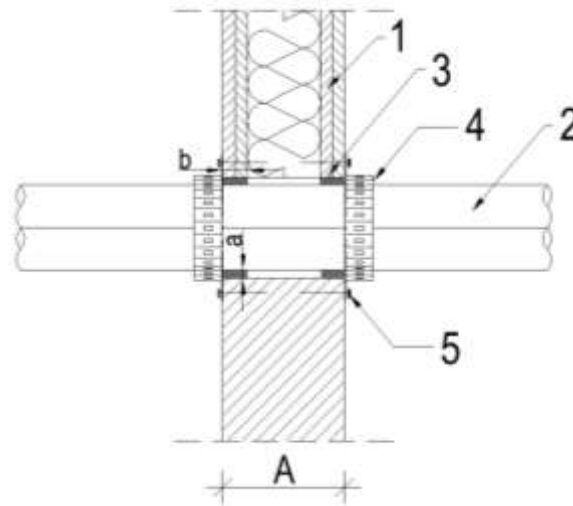
Fig. D5. Plastic conduit bundle penetration seals made with use of INTU FR COLLAR L SLIM collars (double-sided) in flexible or rigid wall
