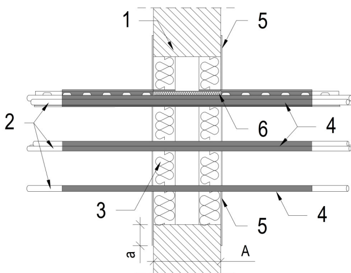
Fig. 6. Cable penetration seal with mineral wool filling
