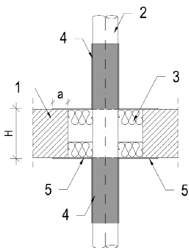
Fig. 4. Filling partition with mineral wool
