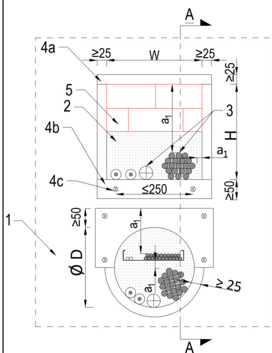
Fig. 2 Cable penetration seal in flexible wall - detail with increased wall thickness
