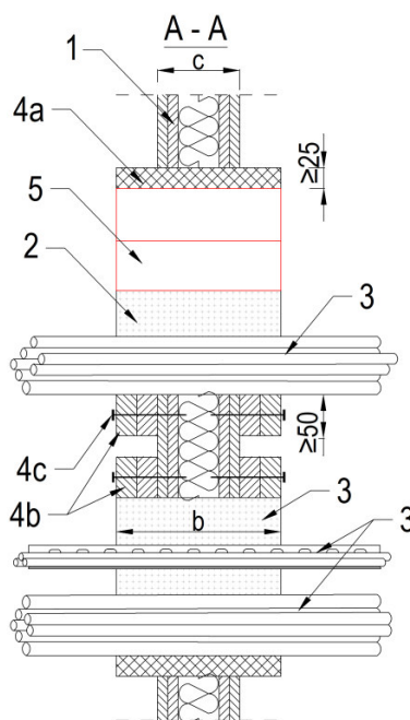
Fig. 2 Cable penetration seal in flexible wall - detail with increased wall thickness
