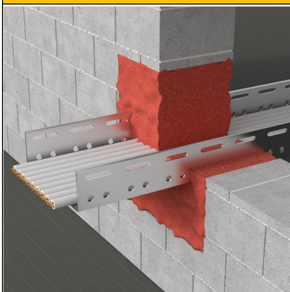
Fig.4 Cable penetration seal in rigid wall
