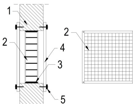
Fig. 1. Installation of INTU FR GRILLE in the wall
